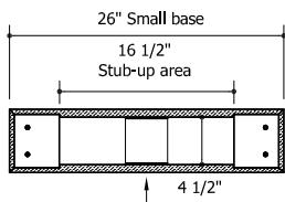
Horizontal section of Small Base
