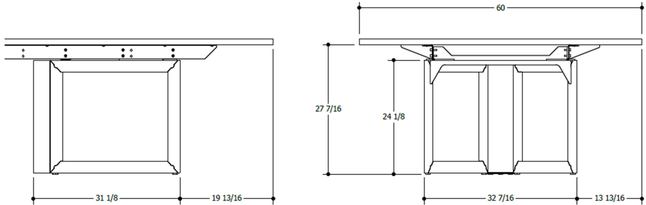
END BASE ELEVATION, 60D
